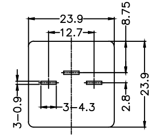
PANEL CUT-OUT(PCB)
